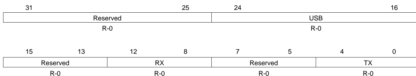
Figure 23. USB Interrupt Mask Register (INTMSKR)
